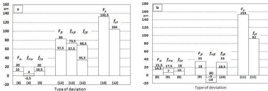
Fig. 2. Maximal and minimal values of the deviations F_\alpha, f_{H\alpha}, f_{f\alpha}, F_\beta, f_{H\beta}, f_{f\beta}, F_p, f_{pt} after hobbing operation: for the LH (a) and RH (b) active flank
