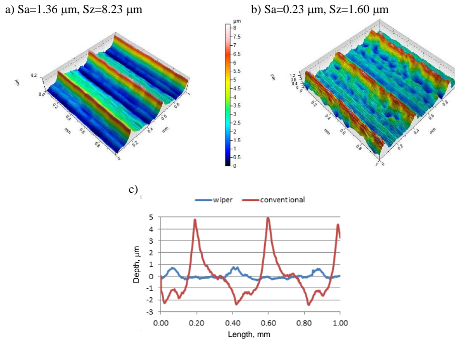
Fig. 6. Surface topographies and surface profiles obtained for feed f = 0,4 \text{ mm} : a) conventional (C), b) wiper (W) and c) difference between surface profiles for C and W tools
