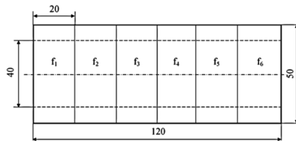
Fig. 2 The sketch of machined workpiece.
