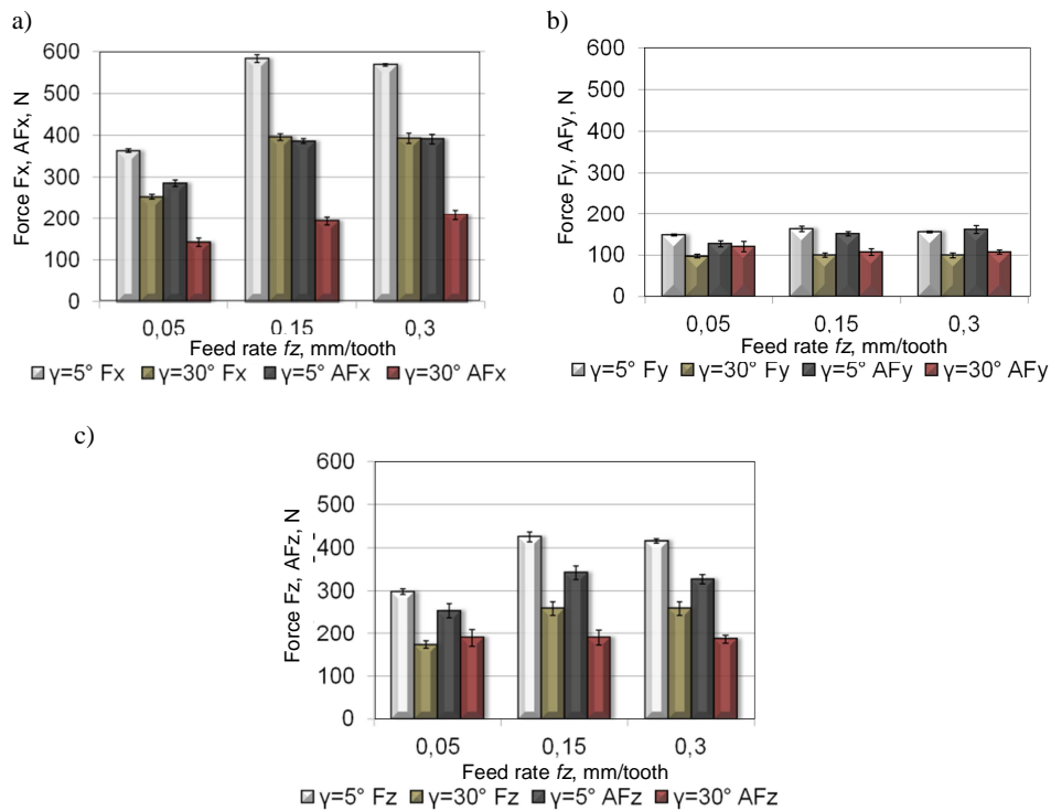
Fig. 3. The effect of change in feed rate per tooth f_z on the value of cutting force components and their amplitudes during milling of AZ91HP magnesium alloy using tools of various rake angles:
